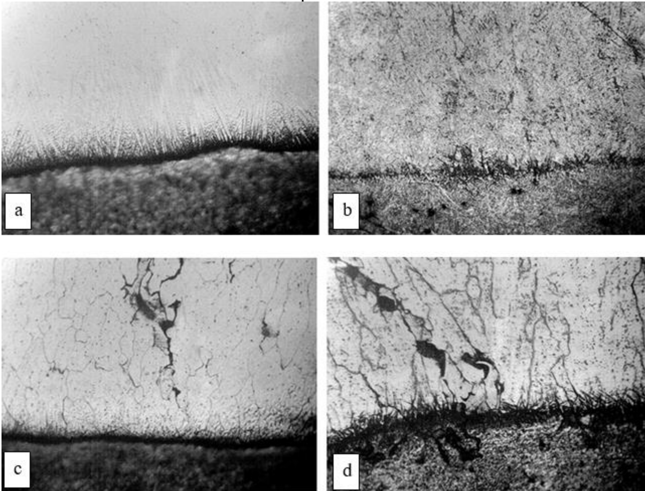
Fig. 1. Microstructure of deposited metal with different boron content (x200): a – without boron; b – 0.007%; c – 0.02%; d – 0.05%
